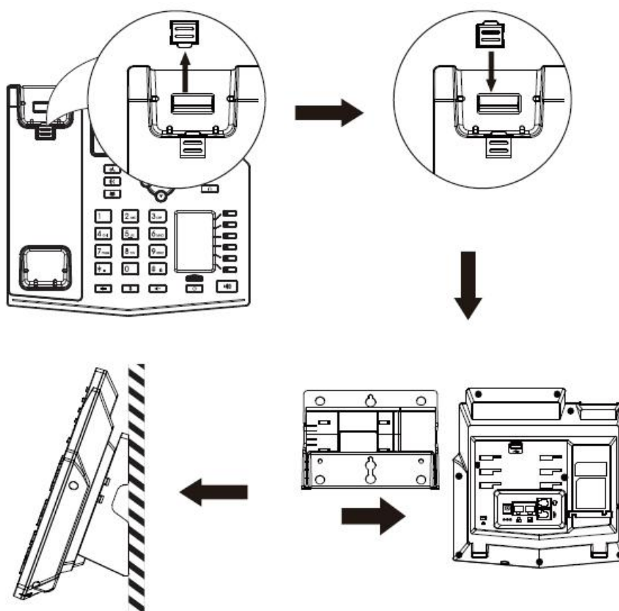
Photo 2 – Installation murale
